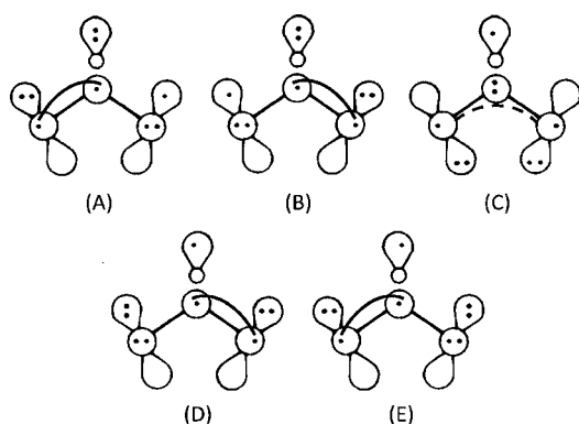
Figure 1. GVB diagrams for NO 2 . (A–C) Three VB diagrams for NO 2 that combine to form the ground state. Here each atom is neutral, and the curved solid lines in (A,B) indicate spin paired π bonds, while the curved dashed line in (C) indicates the four-electron three-center π bond, as in the ozone ground state. Often the neutral diagram (C) is written as the superposition of the zwitterion states shown in (D,E).
