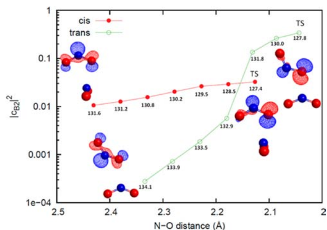
Figure 11. The weighting of B_2 orbital ( |c_{B_2}|^2 ) based on the decomposition of GVB orbital \varphi_{\text{GVB}} = c_{A_1}\varphi_{A_1} + c_{B_2}\varphi_{B_2} as a function of N–O distance to form cis - and trans-ONO-NO}_2 . For trans-ONO-NO}_2 , the much larger |c_{B_2}|^2 at TS indicates that there is more A_1 \rightarrow B_2 excitation involved and hence a higher barrier. The GVB orbital for both cases at reactant side (mostly A_1 ) and TS (mixture of A_1 and B_2 ) is also given. The ONO bond angle is given at each geometry.
